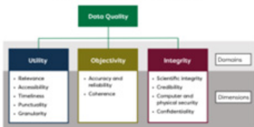
Figure ES 1. The FCSM Data Quality Framework
