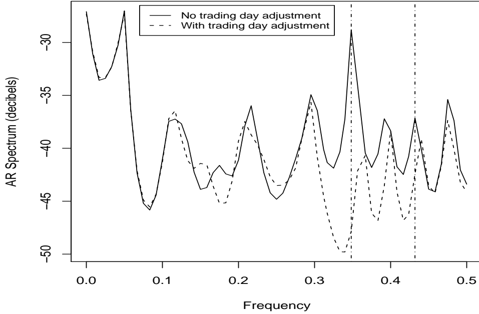
Spectrum of the Differenced Logged Seasonally Adjusted Series Finished Goods Inventories of Primary Metals
