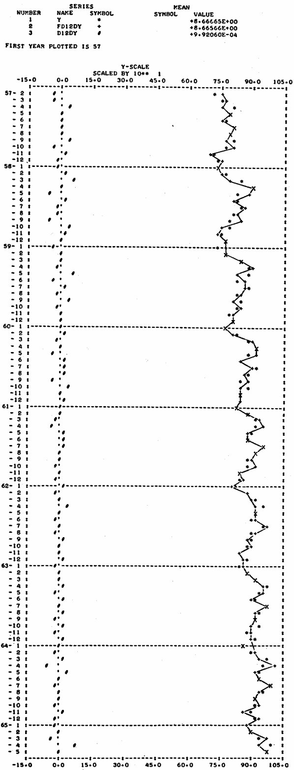
Figure 1. ACTUALS, FITTED NONSTATIONARY, D12DLOGY
