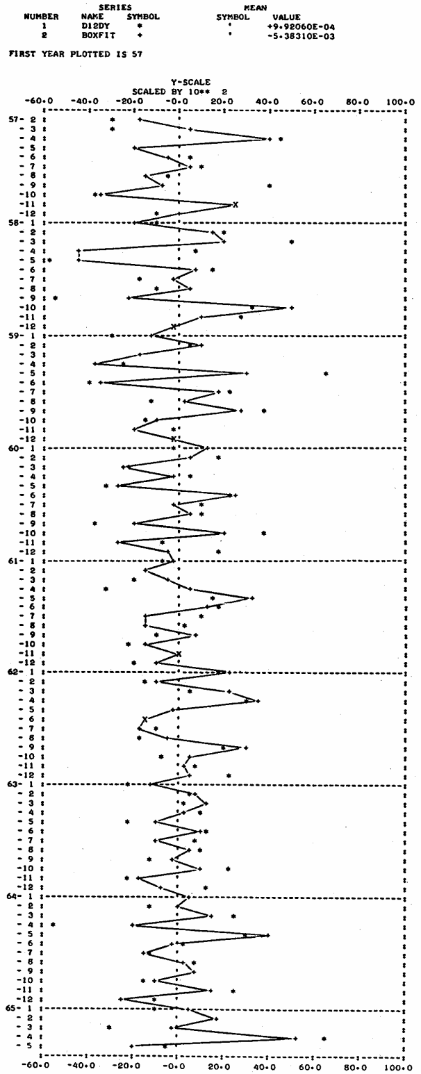
Figure 2. D12DLOGY AND FITTED STATIONARY
